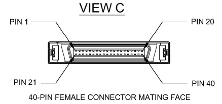
40-PIN FEMALE CONNECTOR MATING FACE
