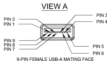
9-PIN FEMALE USB-A MATING FACE
